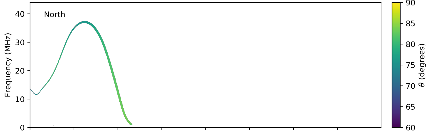
expres_earth_jupiter_europa_jrm09_lossc-wid1deg_3kev_20070906_v01.cdf
