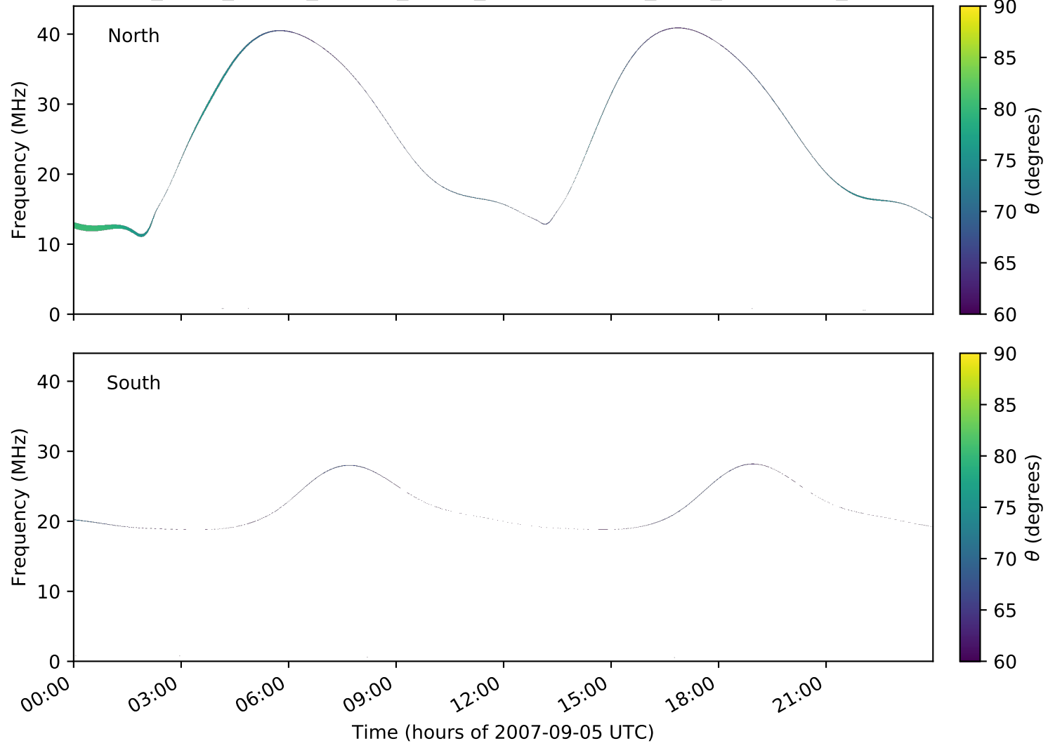
expres_earth_jupiter_europa_jrm09_lossc-wid1deg_3kev_20070905_v01.cdf
