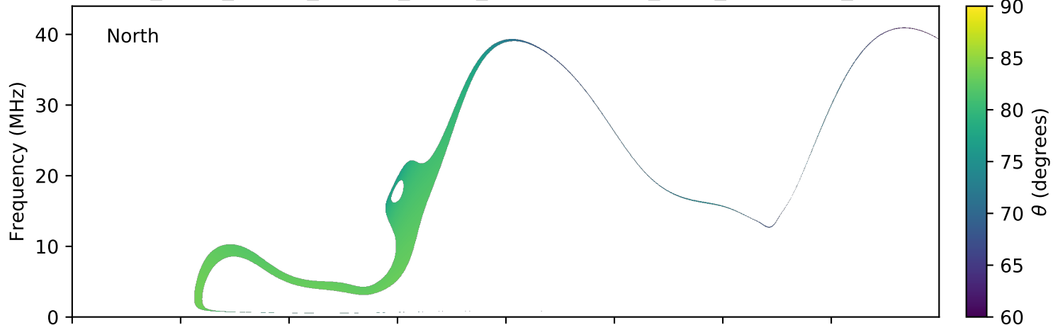
expres_earth_jupiter_europa_jrm09_lossc-wid1deg_3kev_20070901_v01.cdf
