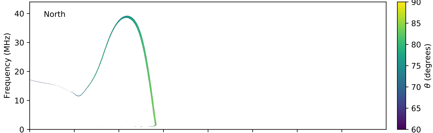
expres_earth_jupiter_io_jrm09_lossc-wid1deg_3kev_20070729_v01.cdf
