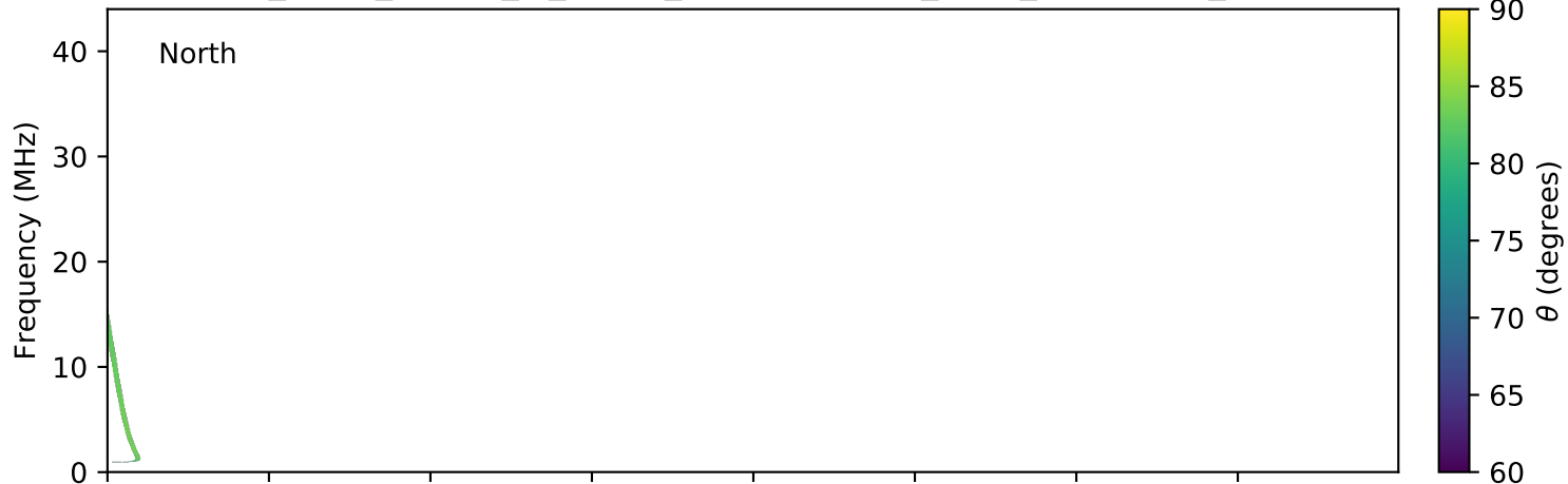
expres_earth_jupiter_io_jrm09_lossc-wid1deg_3kev_20070724_v01.cdf
