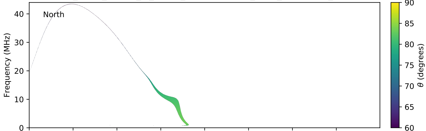
expres_earth_jupiter_io_jrm09_lossc-wid1deg_3kev_20070720_v01.cdf
