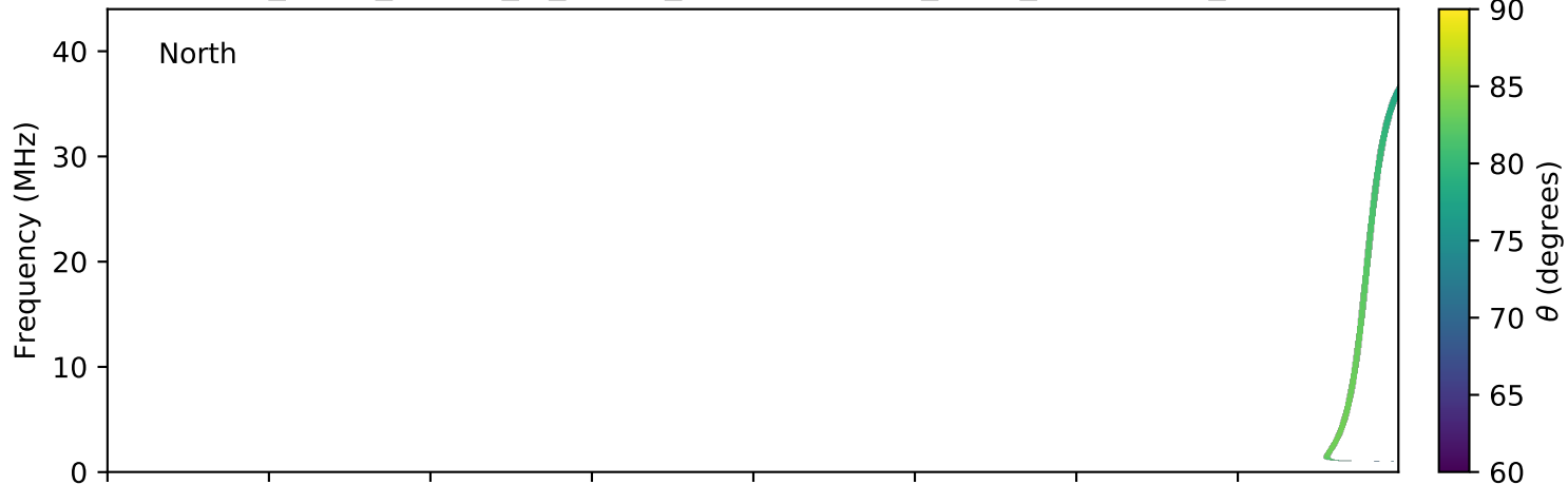
expres_earth_jupiter_io_jrm09_lossc-wid1deg_3kev_20070717_v01.cdf
