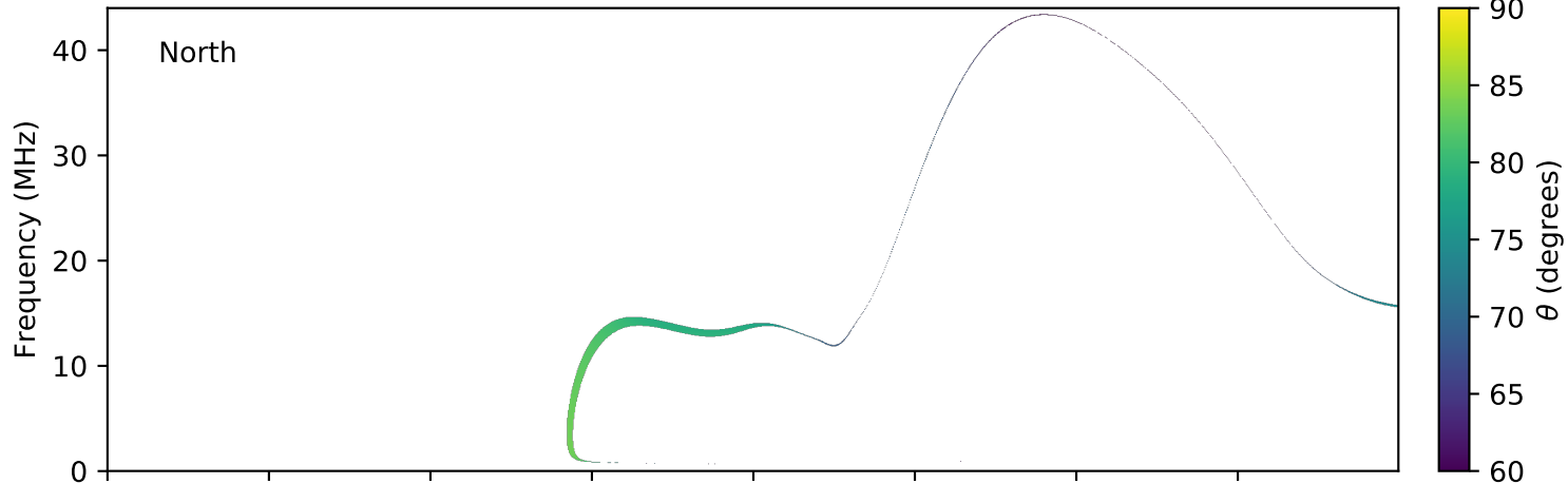
expres_earth_jupiter_io_jrm09_lossc-wid1deg_3kev_20070714_v01.cdf
