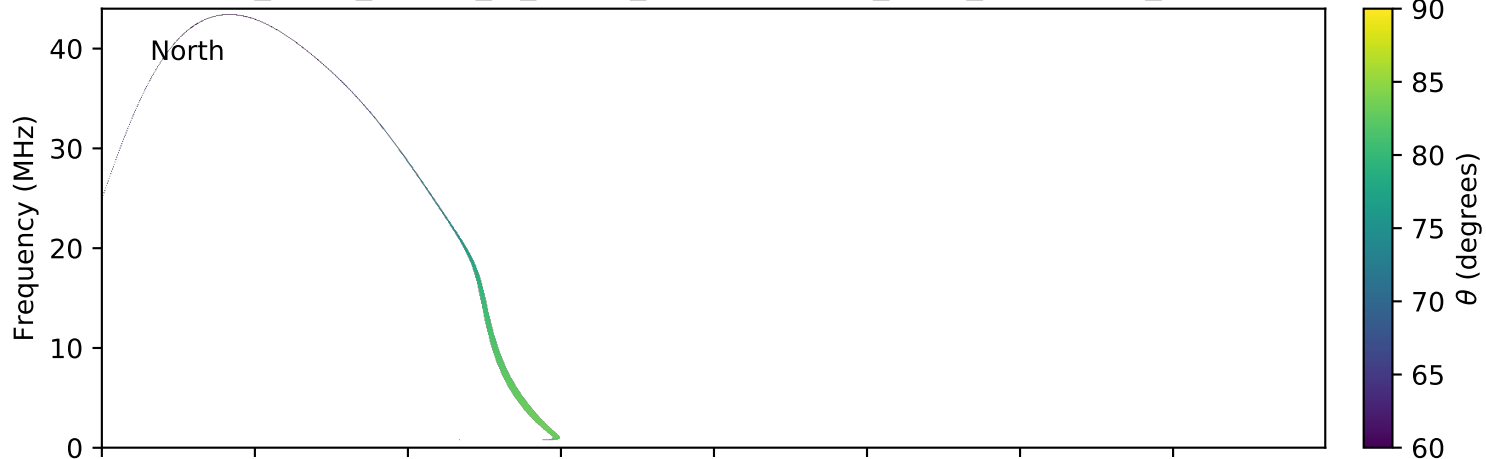
expres_earth_jupiter_io_jrm09_lossc-wid1deg_3kev_20070713_v01.cdf
