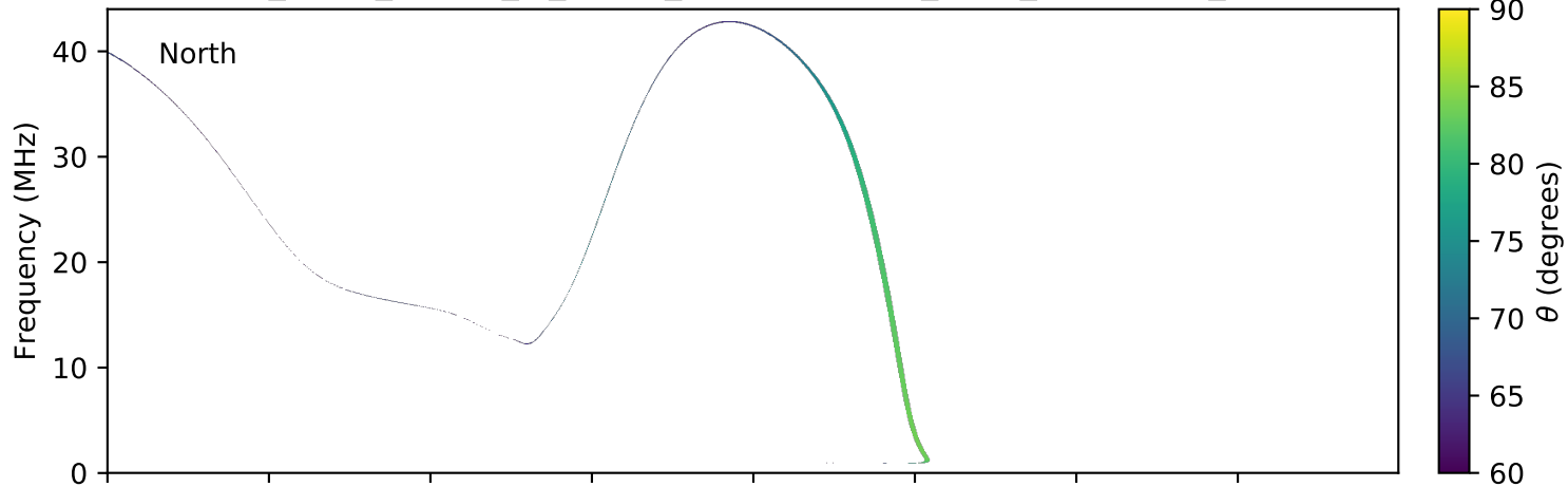
expres_earth_jupiter_io_jrm09_lossc-wid1deg_3kev_20070711_v01.cdf
