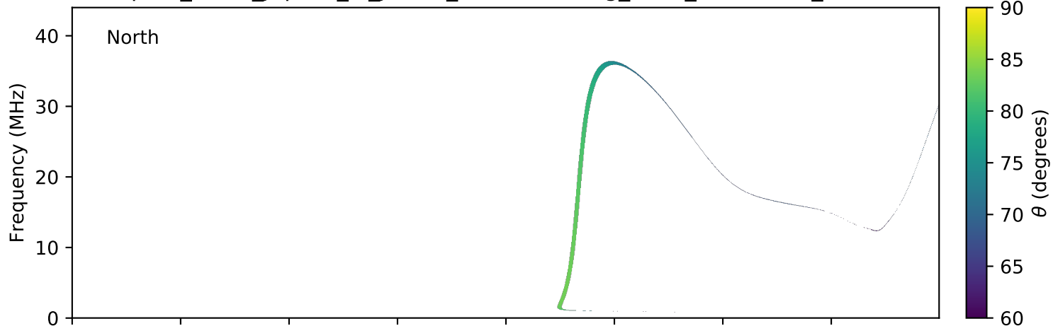
expres_earth_jupiter_io_jrm09_lossc-wid1deg_3kev_20070705_v01.cdf
