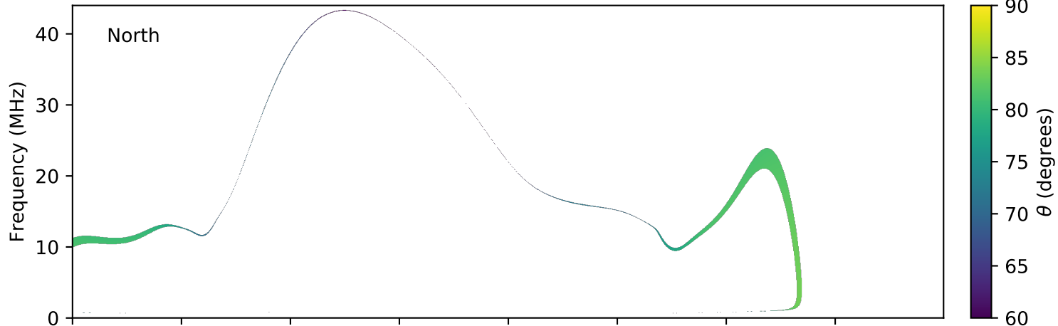
expres_earth_jupiter_io_jrm09_lossc-wid1deg_3kev_20070702_v01.cdf
