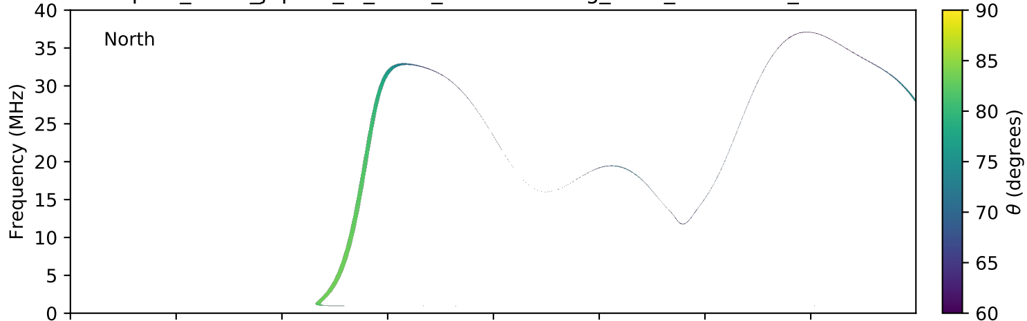
expres_earth_jupiter_io_isaac_lossc-wid1deg_3kev_20070730_v01.cdf
