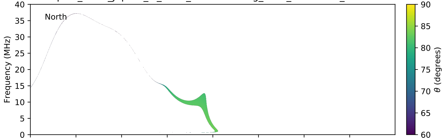
expres_earth_jupiter_io_isaac_lossc-wid1deg_3kev_20070727_v01.cdf
