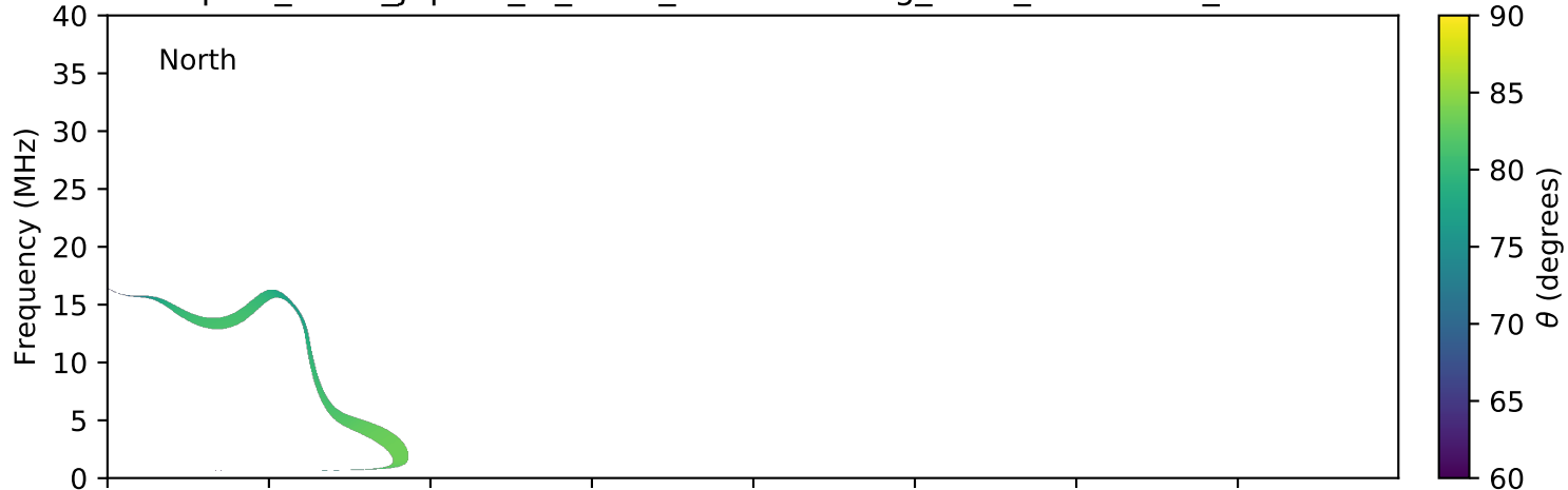
expres_earth_jupiter_io_isaac_lossc-wid1deg_3kev_20070722_v01.cdf
