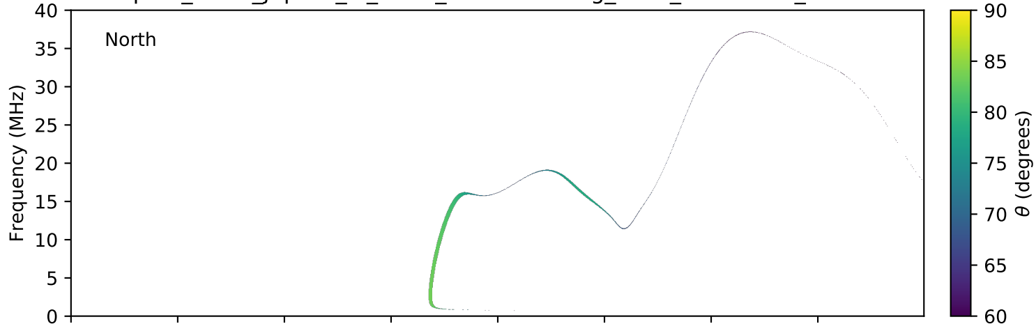
expres_earth_jupiter_io_isaac_lossc-wid1deg_3kev_20070721_v01.cdf
