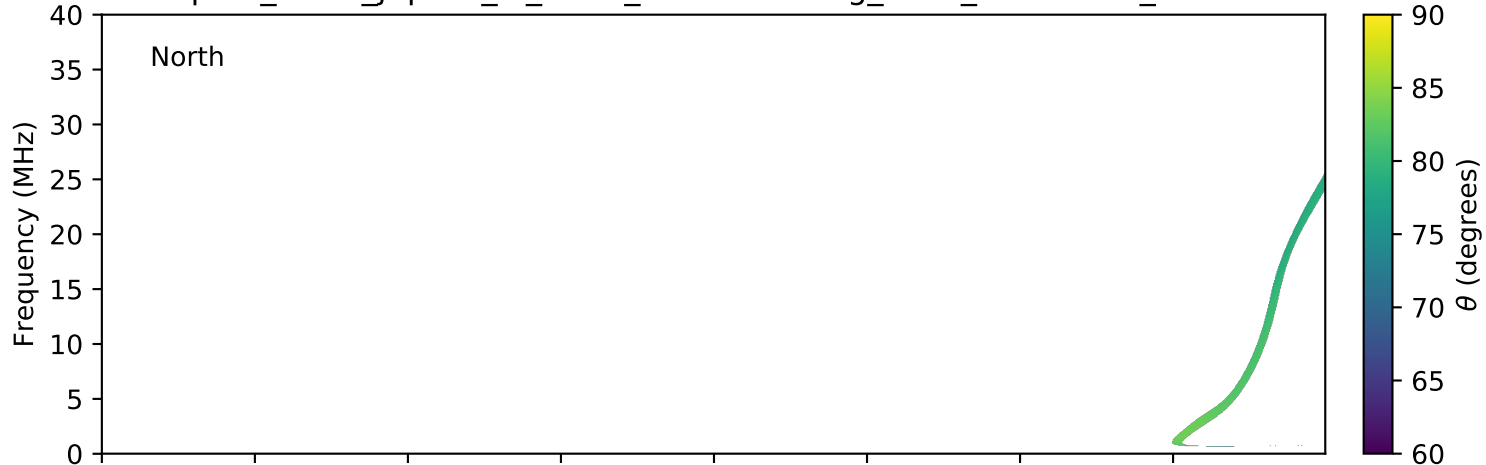
expres_earth_jupiter_io_isaac_lossc-wid1deg_3kev_20070717_v01.cdf
