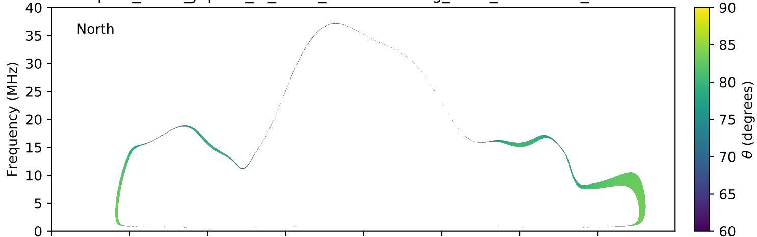
expres_earth_jupiter_io_isaac_lossc-wid1deg_3kev_20070716_v01.cdf
