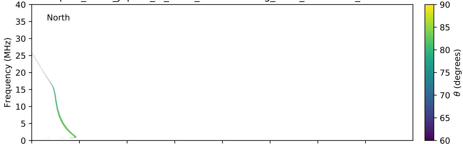
expres_earth_jupiter_io_isaac_lossc-wid1deg_3kev_20070715_v01.cdf
