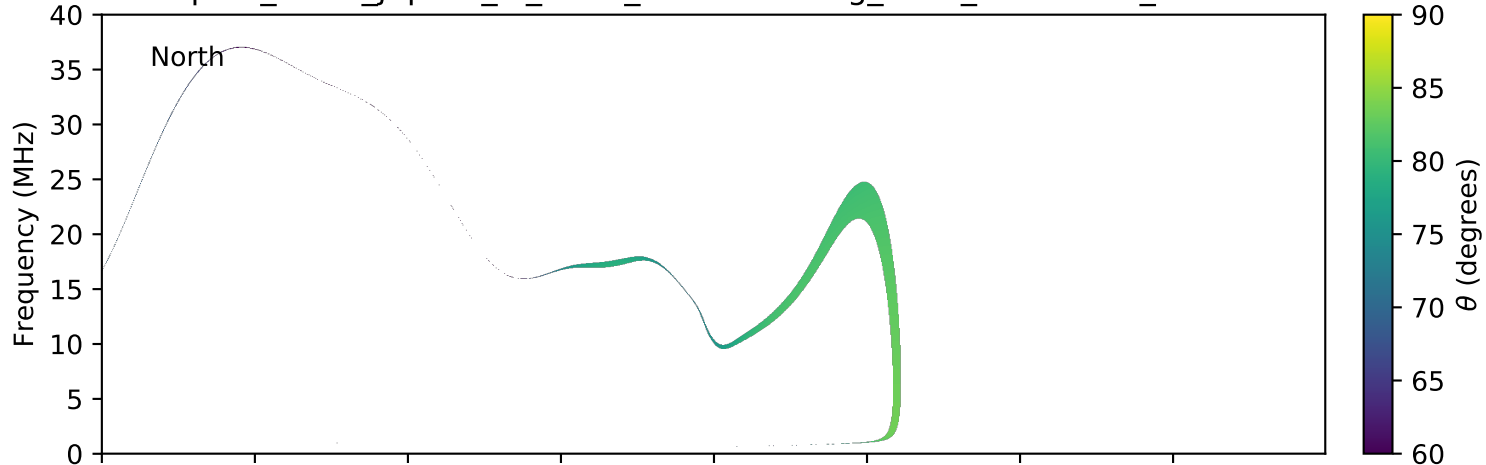
expres_earth_jupiter_io_isaac_lossc-wid1deg_3kev_20070711_v01.cdf
