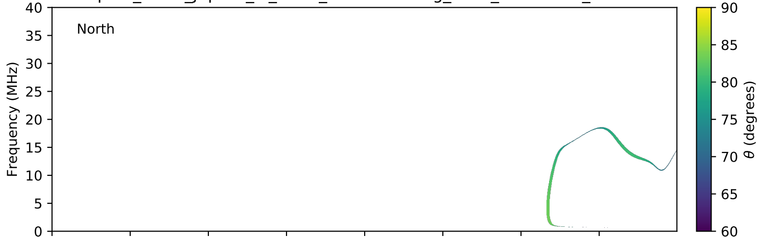
expres_earth_jupiter_io_isaac_lossc-wid1deg_3kev_20070710_v01.cdf
