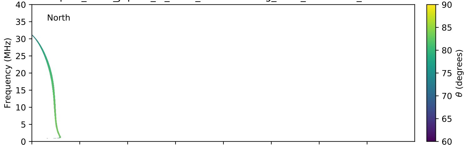
expres_earth_jupiter_io_isaac_lossc-wid1deg_3kev_20070708_v01.cdf
