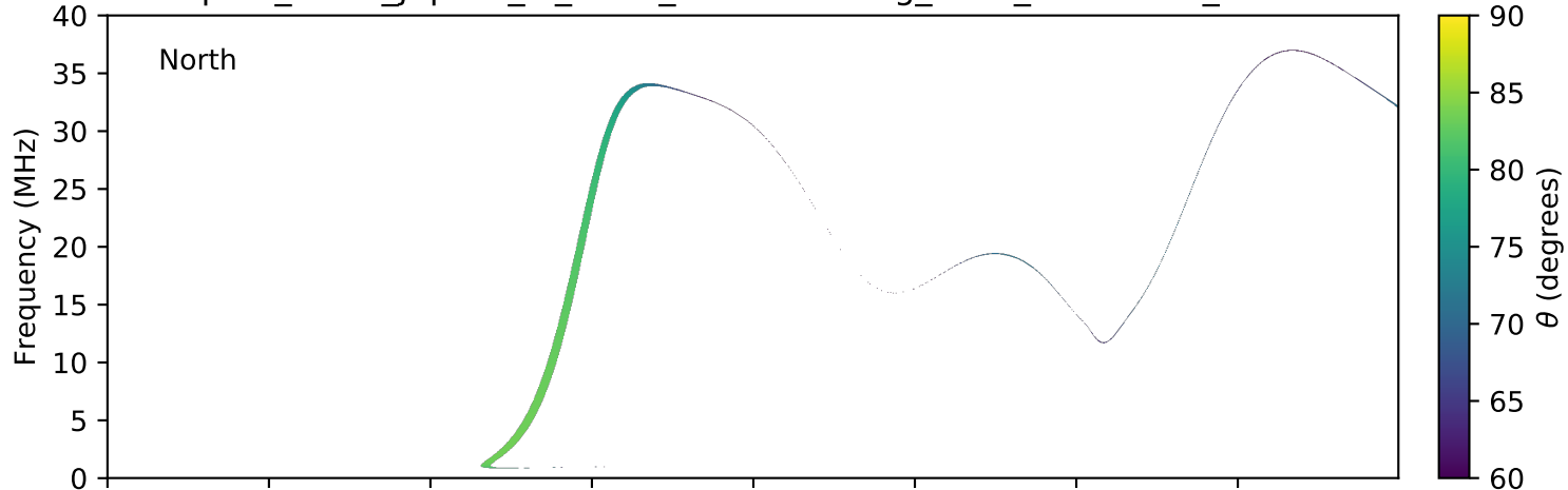
expres_earth_jupiter_io_isaac_lossc-wid1deg_3kev_20070707_v01.cdf
