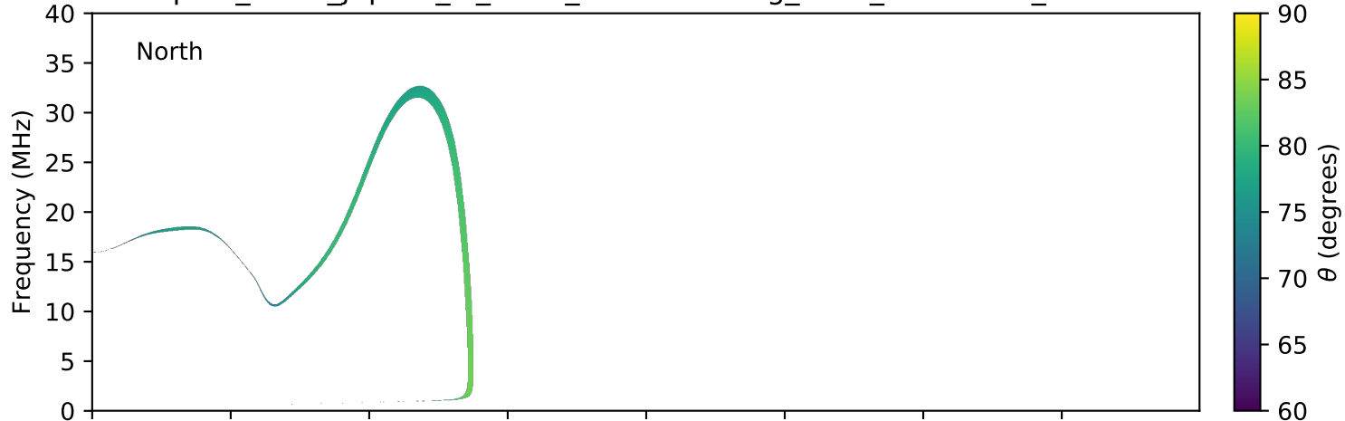
expres_earth_jupiter_io_isaac_lossc-wid1deg_3kev_20070706_v01.cdf
