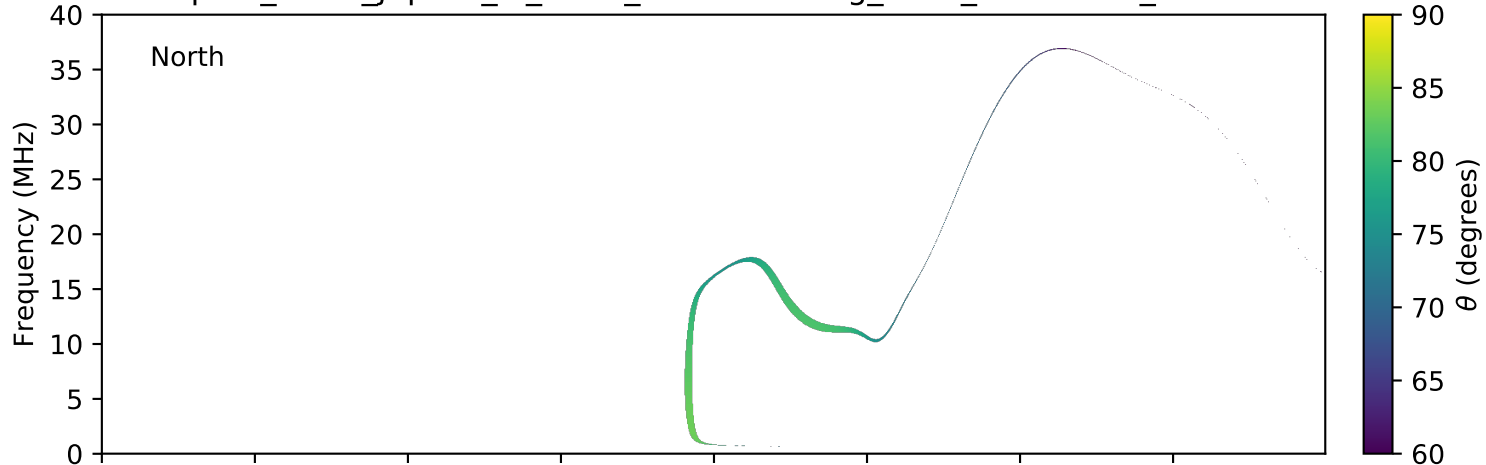
expres_earth_jupiter_io_isaac_lossc-wid1deg_3kev_20070705_v01.cdf
