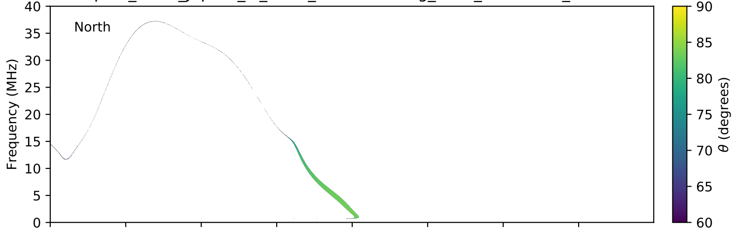
expres_earth_jupiter_io_isaac_lossc-wid1deg_3kev_20070704_v01.cdf
