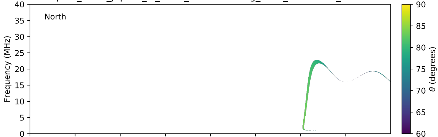
expres_earth_jupiter_io_isaac_lossc-wid1deg_3kev_20070703_v01.cdf
