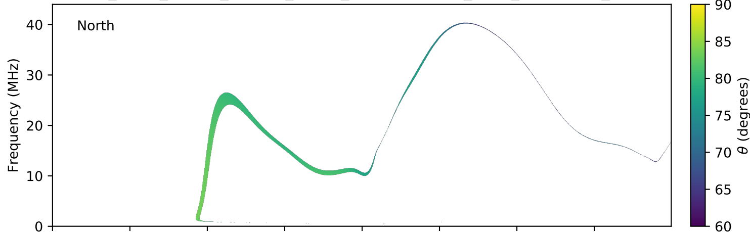
expres_earth_jupiter_europa_jrm09_lossc-wid1deg_3kev_20070731_v01.cdf
