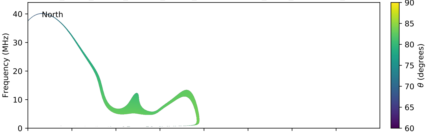
expres_earth_jupiter_europa_jrm09_lossc-wid1deg_3kev_20070704_v01.cdf
