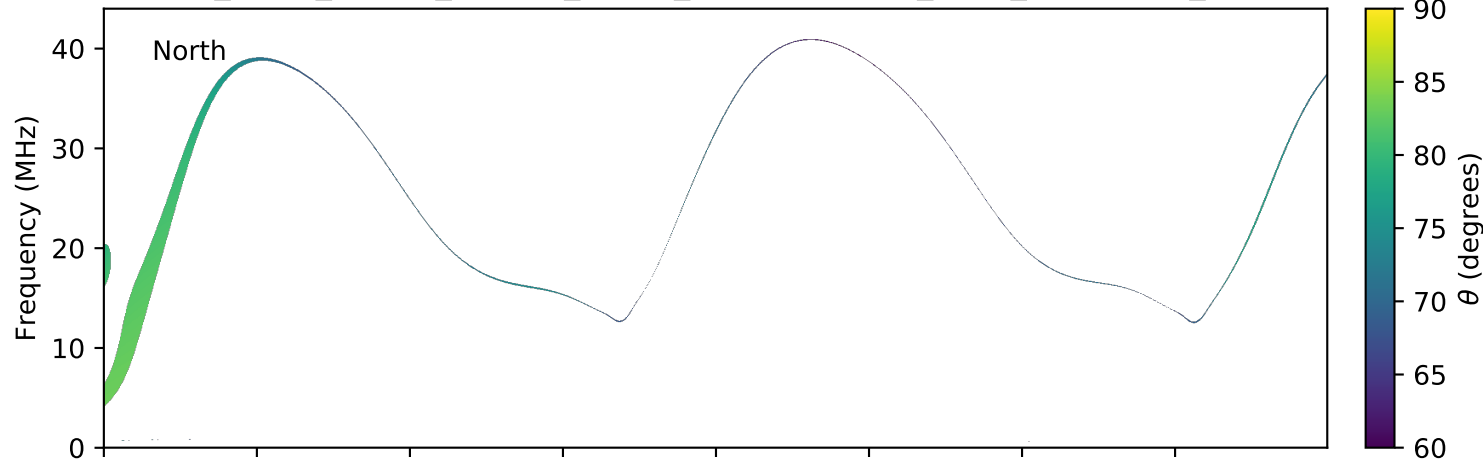
expres_earth_jupiter_europa_jrm09_lossc-wid1deg_3kev_20070703_v01.cdf
