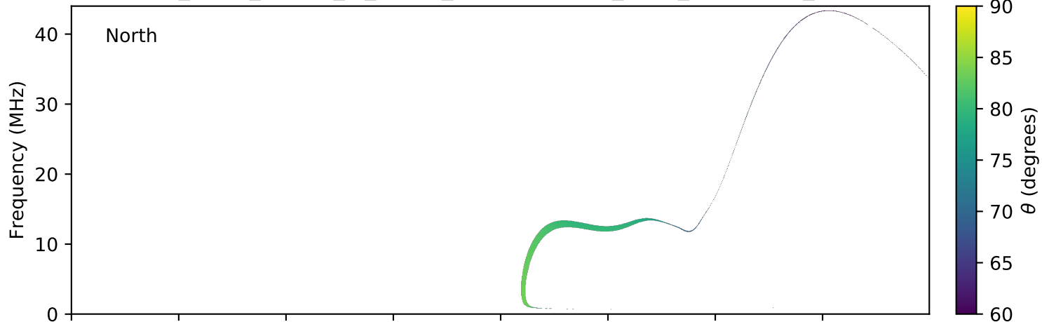
expres_earth_jupiter_io_jrm09_lossc-wid1deg_3kev_20070612_v01.cdf
