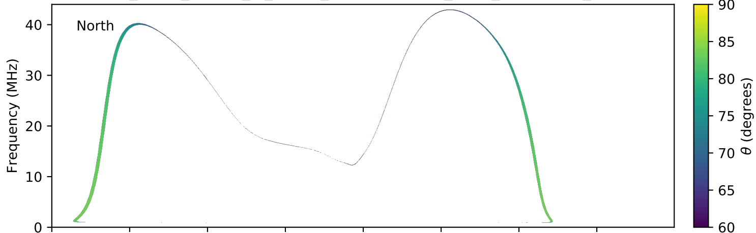
expres_earth_jupiter_io_jrm09_lossc-wid1deg_3kev_20070609_v01.cdf
