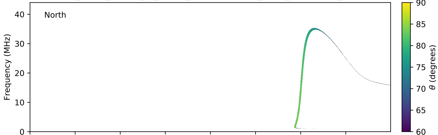
expres_earth_jupiter_io_jrm09_lossc-wid1deg_3kev_20070603_v01.cdf
