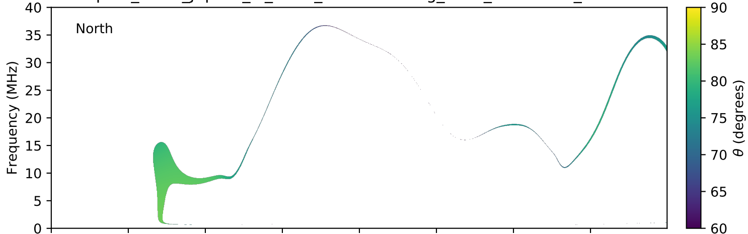
expres_earth_jupiter_io_isaac_lossc-wid1deg_3kev_20070630_v01.cdf
