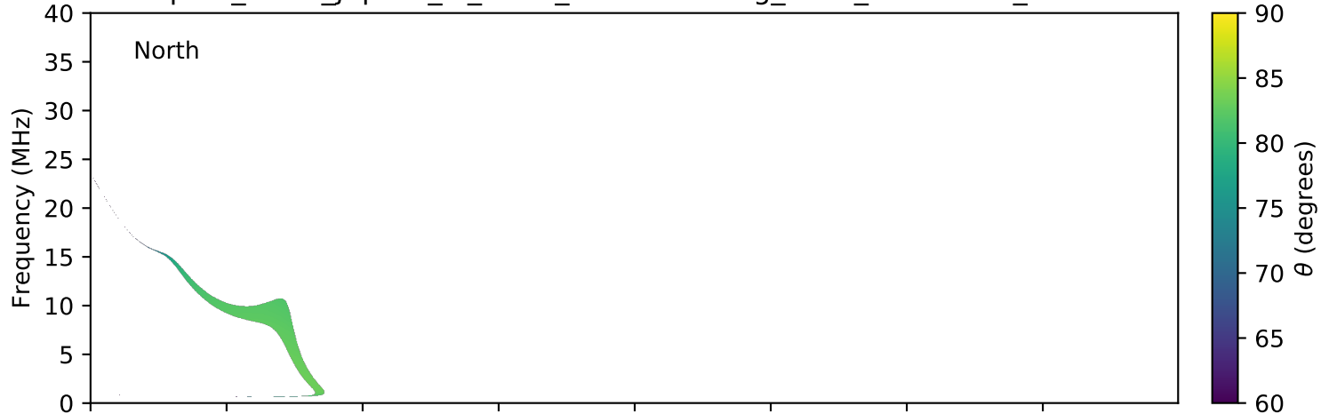
expres_earth_jupiter_io_isaac_lossc-wid1deg_3kev_20070629_v01.cdf
