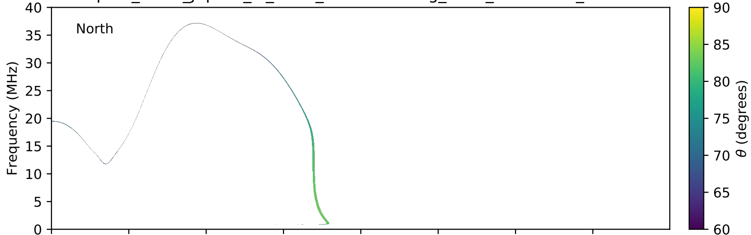
expres_earth_jupiter_io_isaac_lossc-wid1deg_3kev_20070627_v01.cdf
