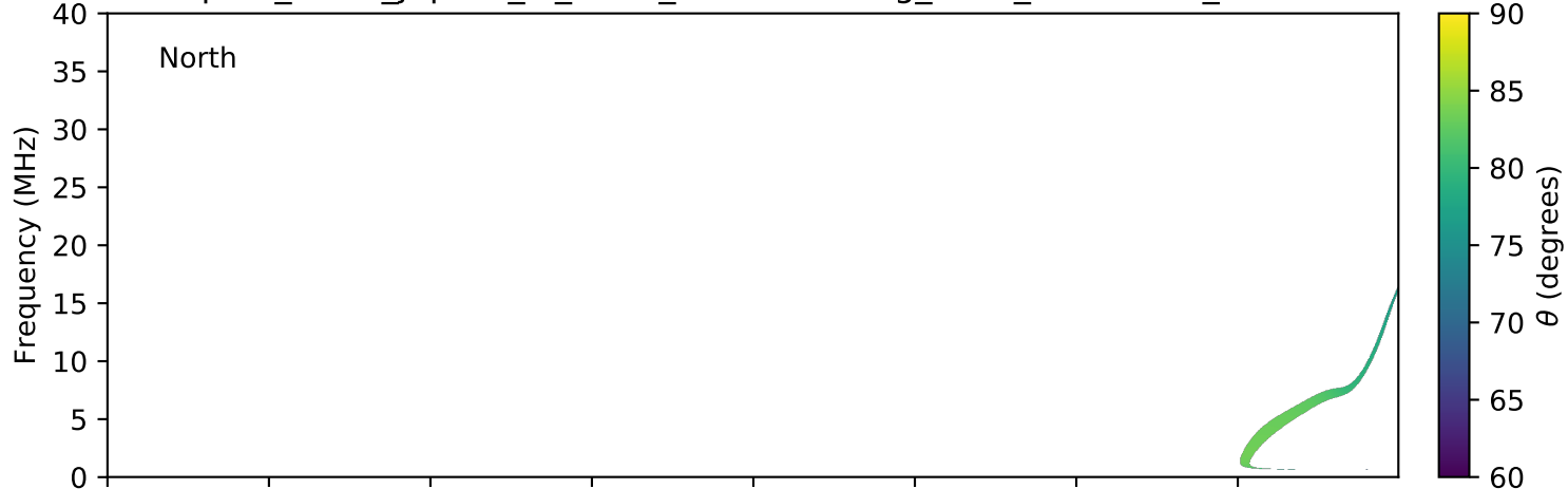
expres_earth_jupiter_io_isaac_lossc-wid1deg_3kev_20070624_v01.cdf
