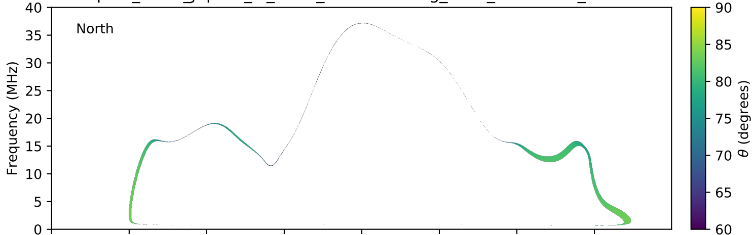
expres_earth_jupiter_io_isaac_lossc-wid1deg_3kev_20070623_v01.cdf
