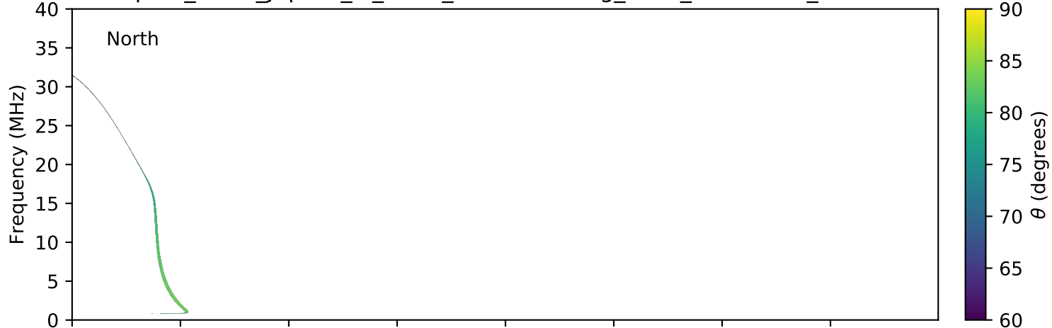
expres_earth_jupiter_io_isaac_lossc-wid1deg_3kev_20070622_v01.cdf
