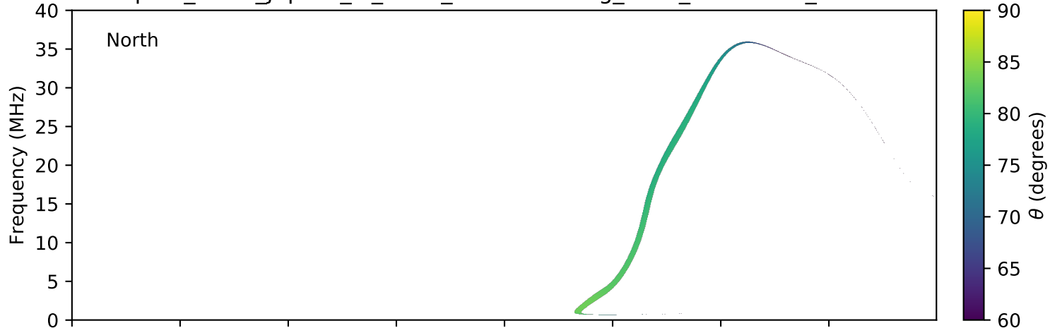
expres_earth_jupiter_io_isaac_lossc-wid1deg_3kev_20070619_v01.cdf
