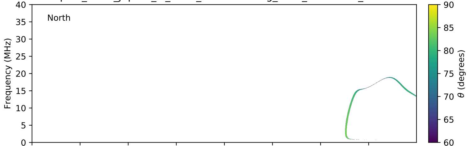
expres_earth_jupiter_io_isaac_lossc-wid1deg_3kev_20070617_v01.cdf
