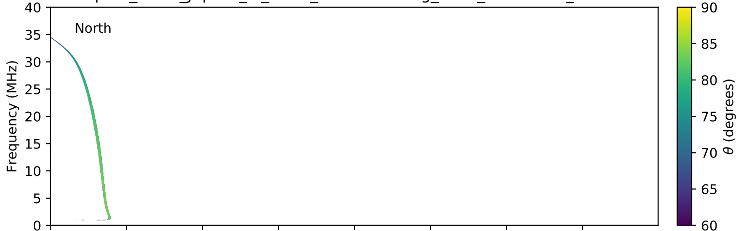
expres_earth_jupiter_io_isaac_lossc-wid1deg_3kev_20070615_v01.cdf
