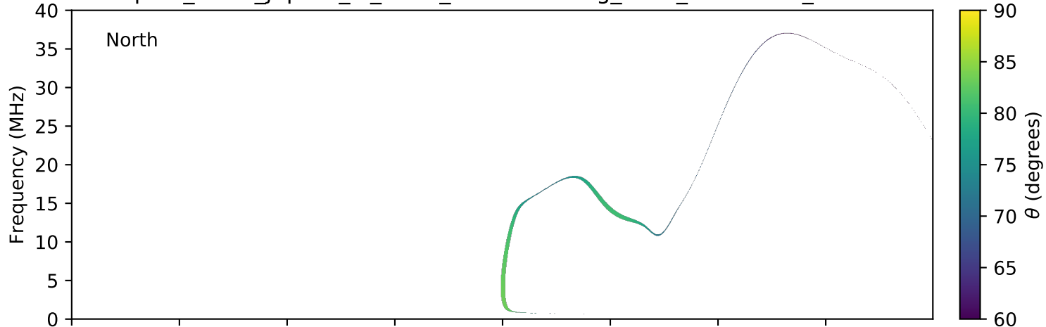
expres_earth_jupiter_io_isaac_lossc-wid1deg_3kev_20070612_v01.cdf
