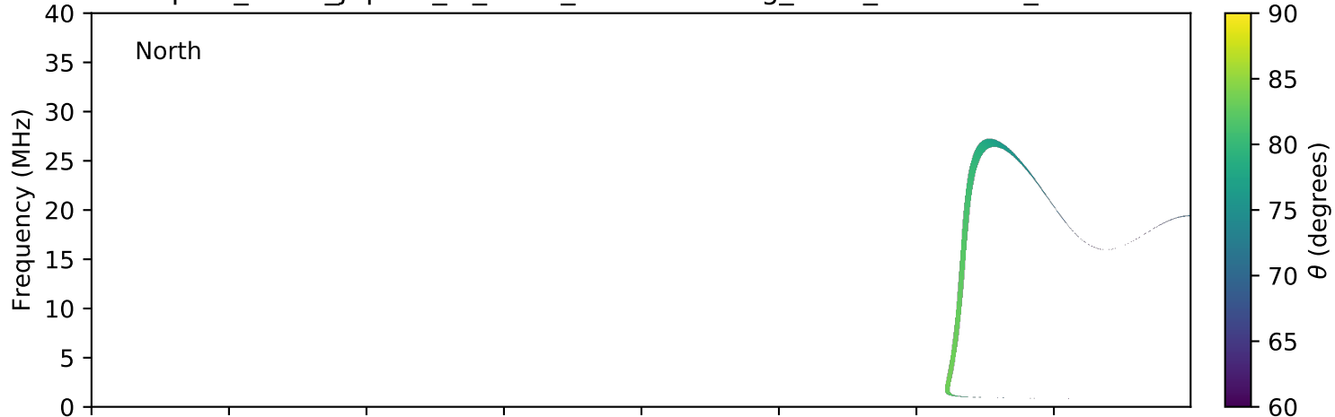
expres_earth_jupiter_io_isaac_lossc-wid1deg_3kev_20070610_v01.cdf
