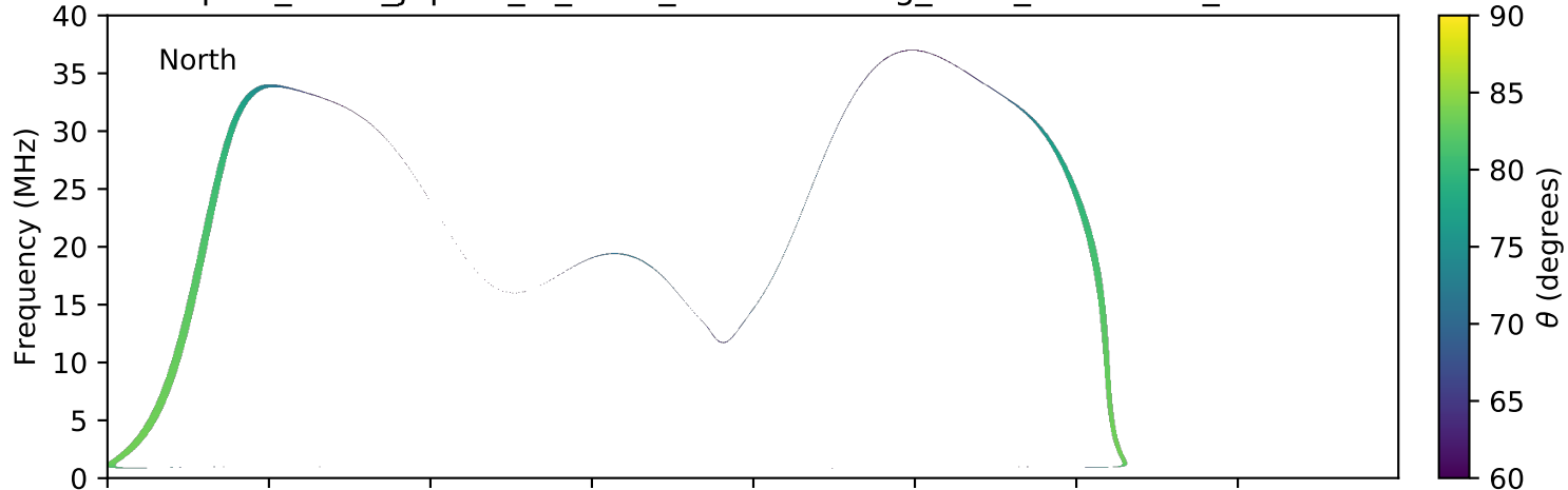
expres_earth_jupiter_io_isaac_lossc-wid1deg_3kev_20070609_v01.cdf
