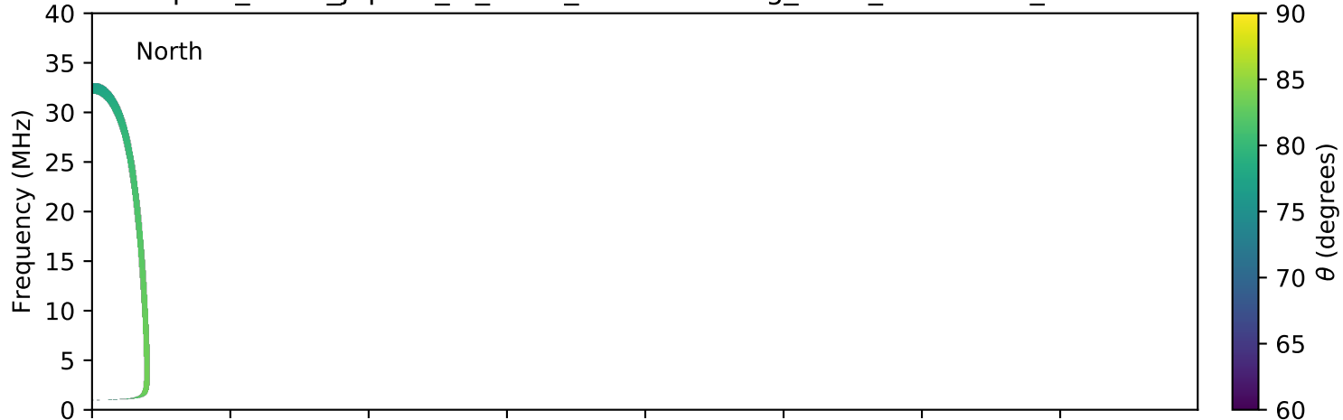
expres_earth_jupiter_io_isaac_lossc-wid1deg_3kev_20070608_v01.cdf
