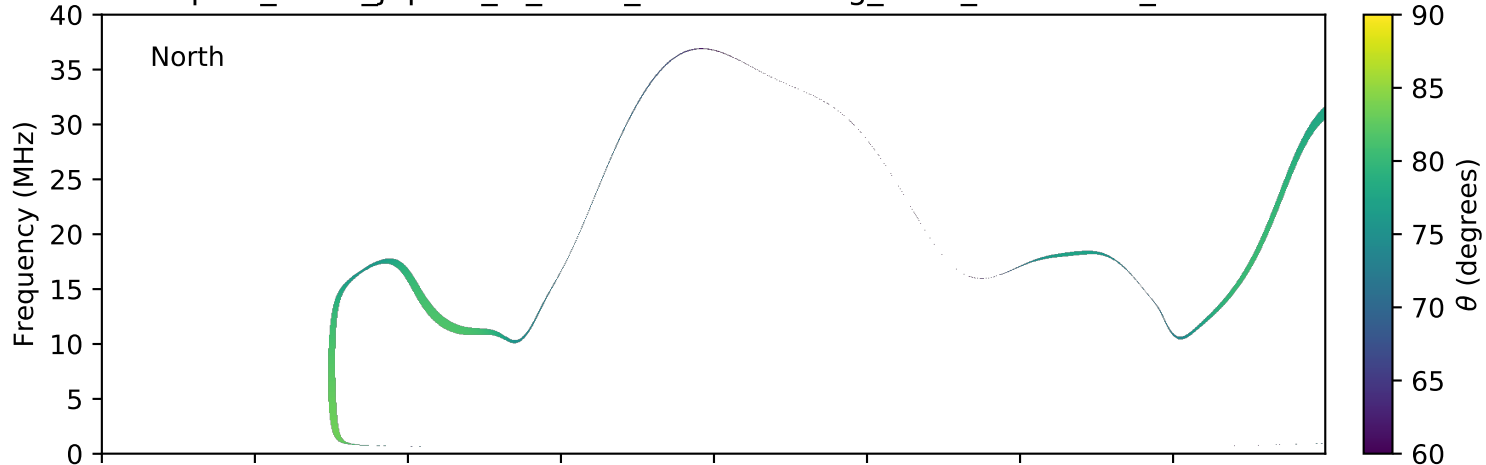
expres_earth_jupiter_io_isaac_lossc-wid1deg_3kev_20070607_v01.cdf
