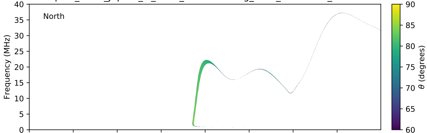
expres_earth_jupiter_io_isaac_lossc-wid1deg_3kev_20070605_v01.cdf
