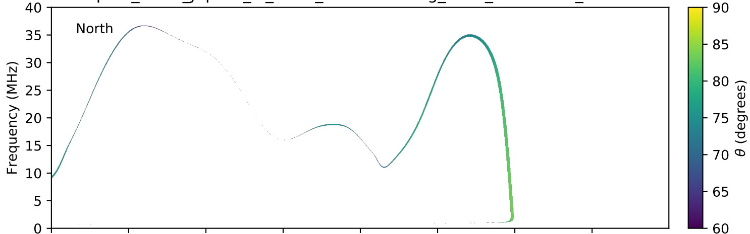
expres_earth_jupiter_io_isaac_lossc-wid1deg_3kev_20070602_v01.cdf
