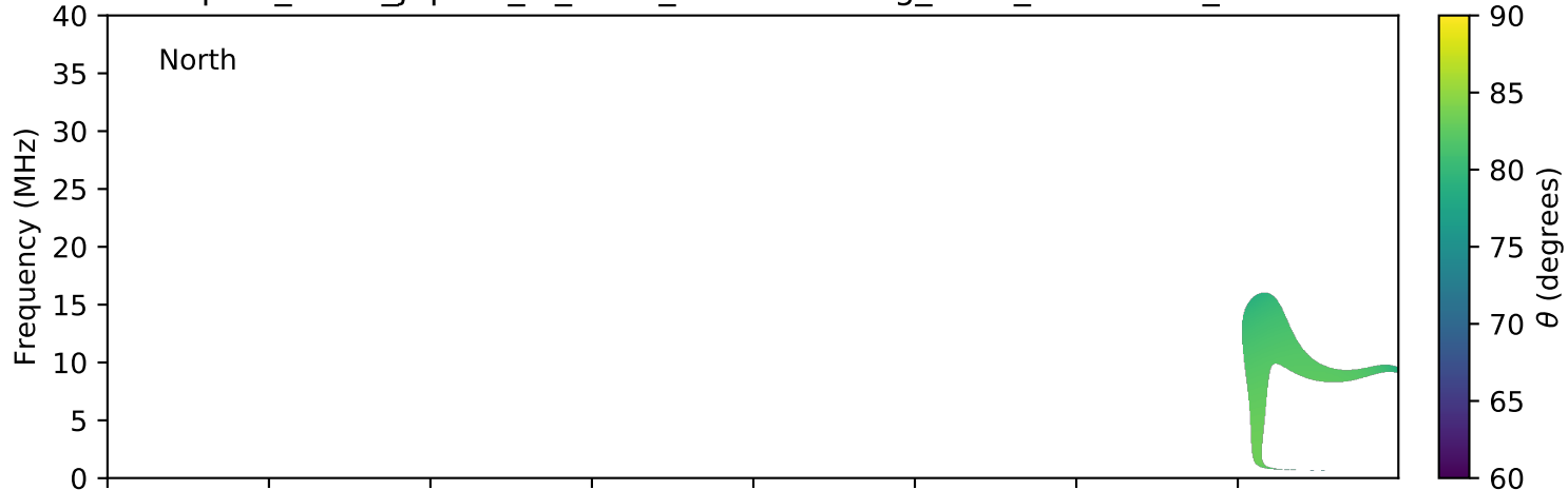
expres_earth_jupiter_io_isaac_lossc-wid1deg_3kev_20070601_v01.cdf
